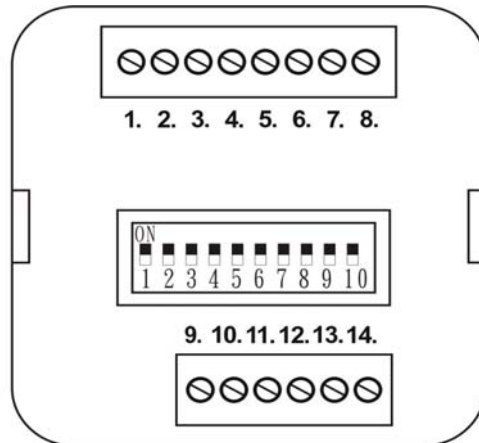
Fig. 2 GTR-17 Controller Back Panel
