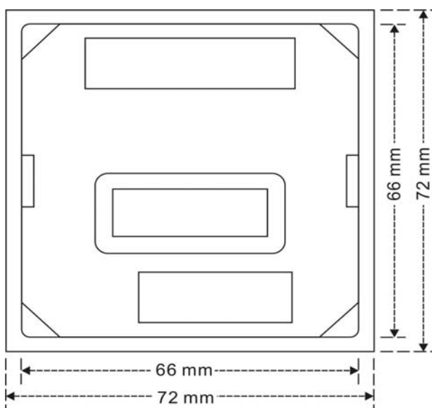
Fig. 3 GTR-17 Case Dimension of Back View
