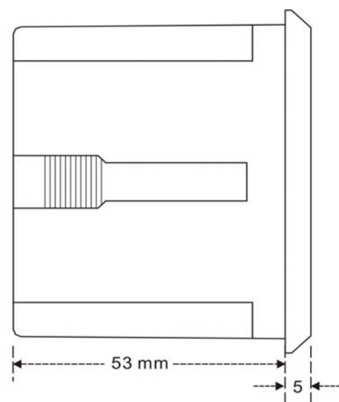
Fig. 4 GTR-17 Case Dimension of Side View
