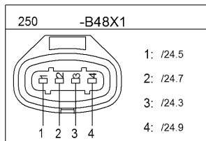
Sensor Boost air
