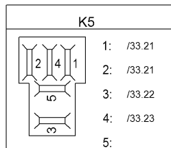
K5: Driving light
