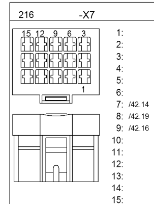
Wire harness Engine room
