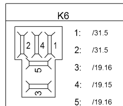
K6: Parking brake
