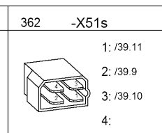
Interface Speedometer mounting
