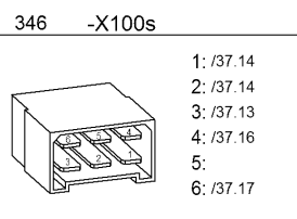
Windshield wiper, front
