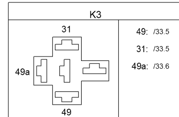
K3: Flasher relay
