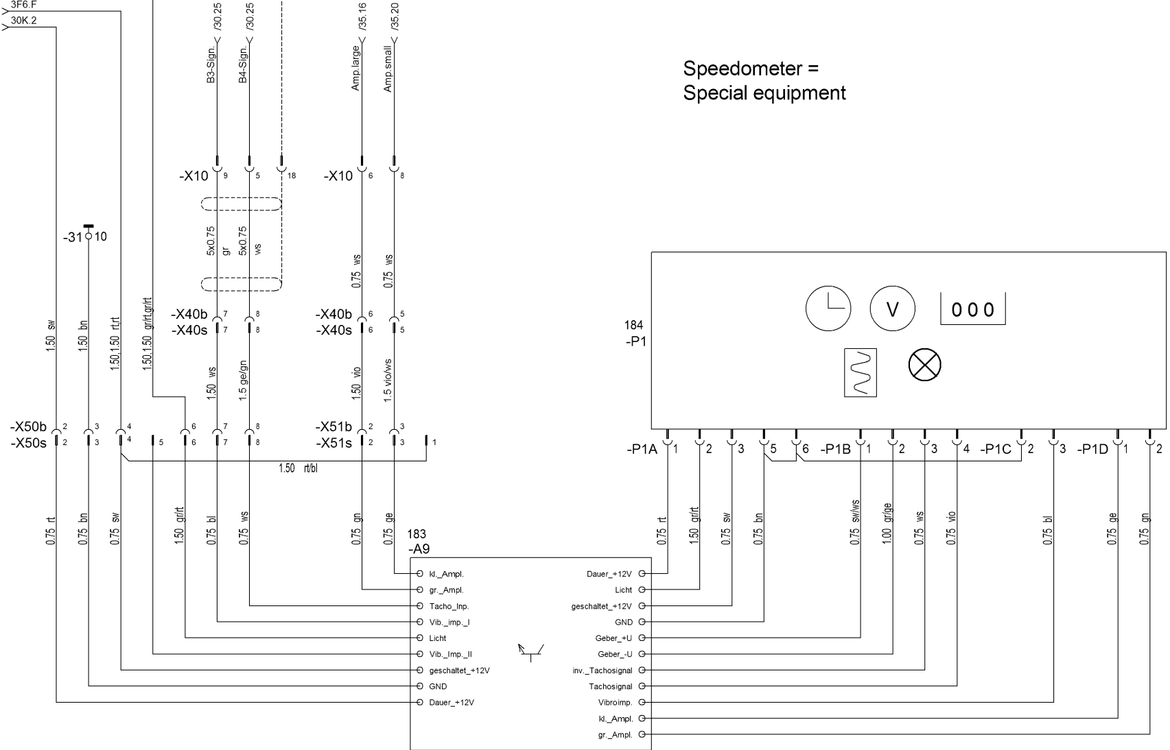
A9: Interface Speedometer
