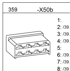
Interface Speedometer mounting
