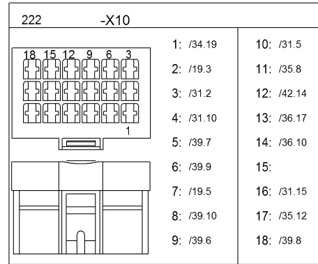
Wire harness Cabin
