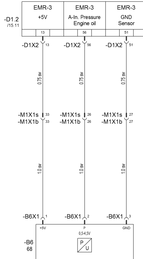
B6: Sensor Engine oil pressure
