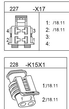
Wire harness high current relay Supply system
