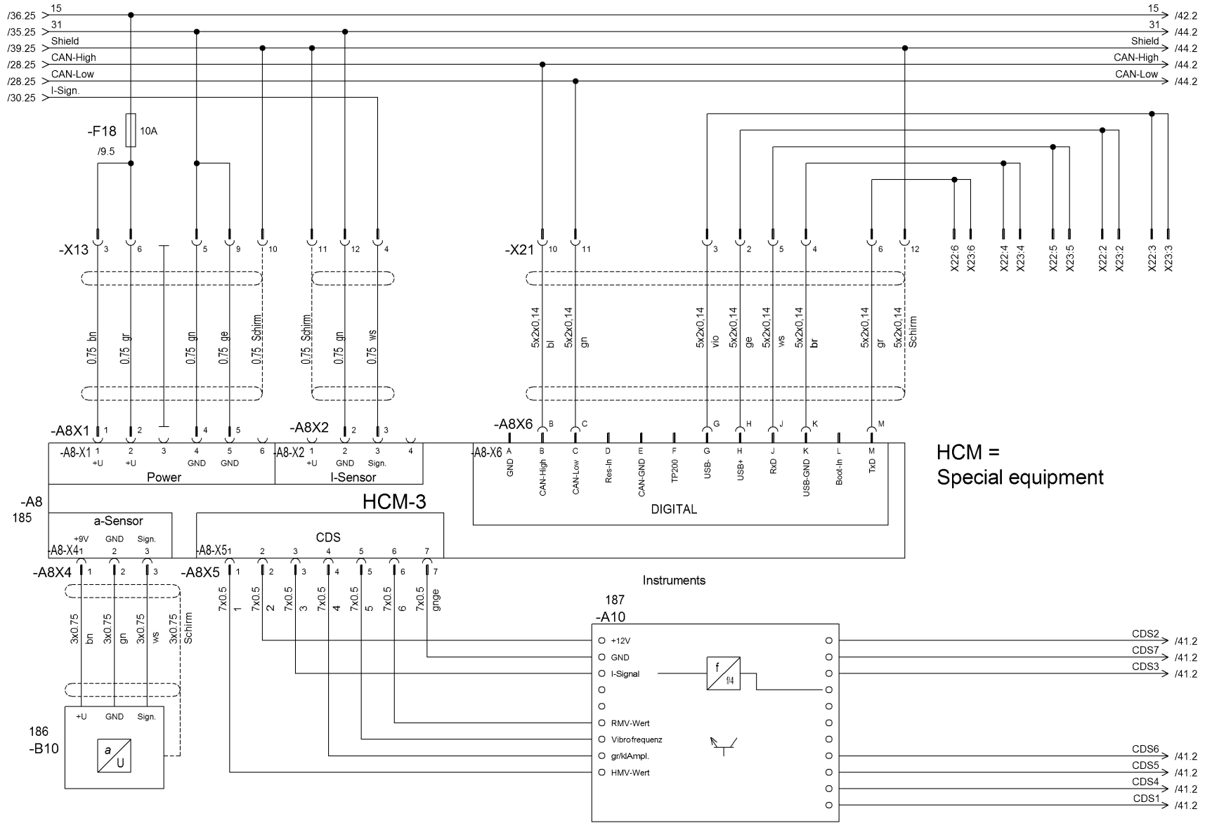
B10: Acceleration sensor
