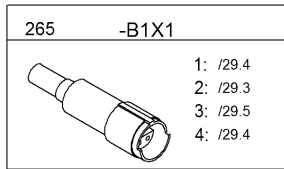
Level transmitter Fuel
