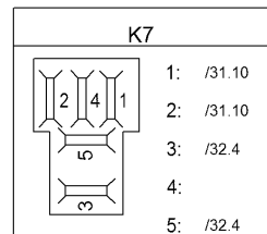
K7: Back-up alarm
