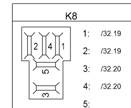
K8: Blade
