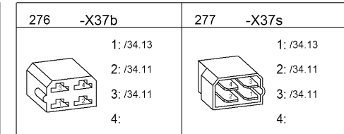
Lighting rear, left
