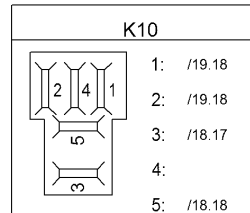
K10: Starting release
