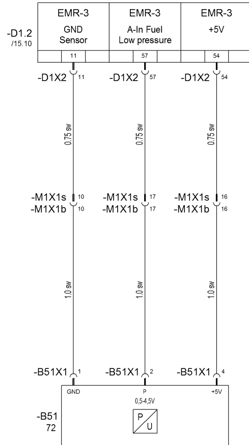
B51: Pressure sensor Fuel Low pressure
