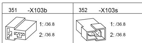
Working spotlights, front right
