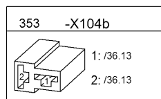
Working spotlights, rear left
