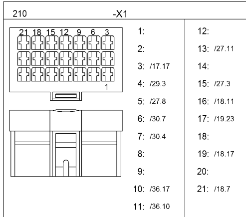
Wire harness Instrument panel
