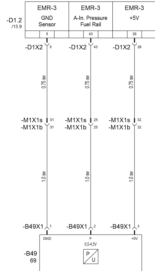
B49: Pressure sensor Fuel Rail
