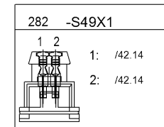
Pressure switch Air conditioning
