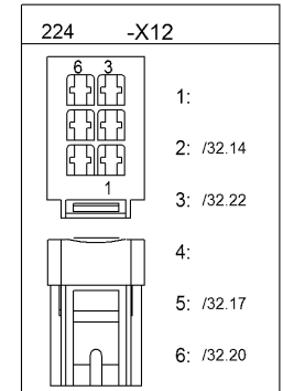
Wire harness Blade
