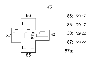
K2: Fuel preheating
