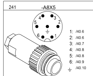
HCM CDS Electric plug
