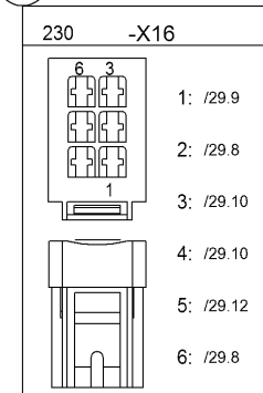
Control device Refuel pump
