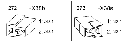
Back-up alarm
