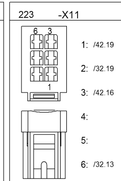
Wire harness Cabin
