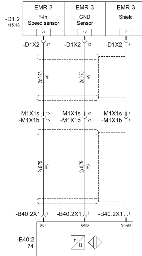
B40.2: Speed sensor Crankshaft
