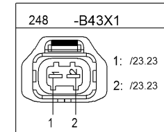
Temperature sensor Coolant
