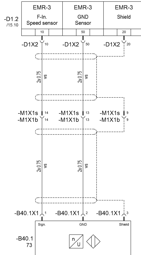
B40.1: Speed sensor Camshaft
