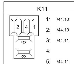
K11: Pilot light Preheat
