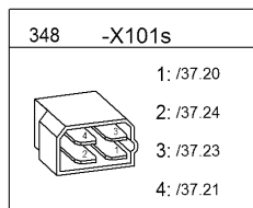
Windshield wiper, rear
