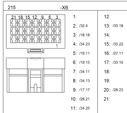
Wire harness Engine room
