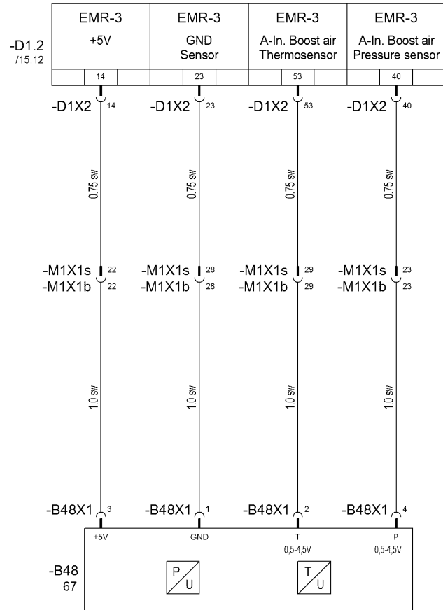
B48: Sensor charge-air pressure / Boost air Thermosensor
