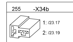
Reserve Starting relay
