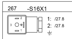
Filter indicator Hydraulic oil filter
