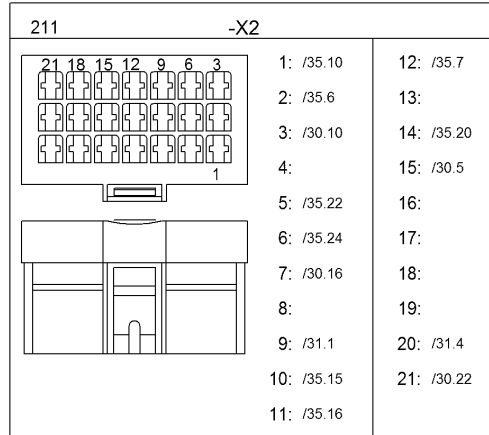
Wire harness Instrument panel
