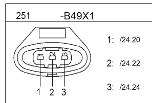
Pressure sensor Fuel RAIL
