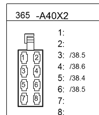
Radio Loudspeaker
