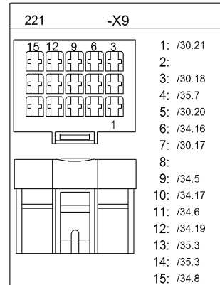
Wire harness Front roller
