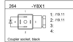
Sensor Coolant level
