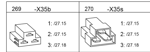
Sensor Coolant level
