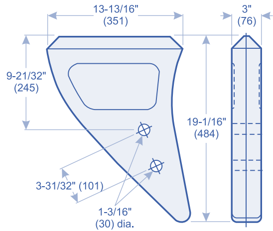
195-78-71380HX 126.0 lbs. (57.1 kgs.)
