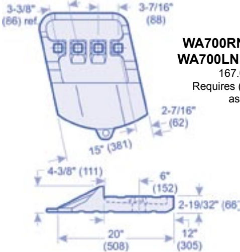
WA700CNR (WA700) 163.0 lbs. (74.0 kgs.) Requires (4) A114-412 plow bolt assemblies each
