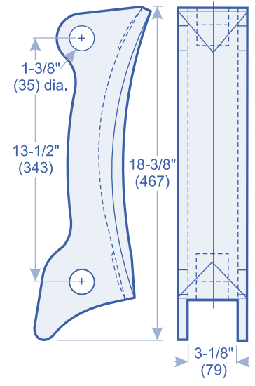
195-78-21320HX 33.6 lbs. (15.3 kgs.)
