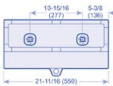
421-815-2211NRHX 88.0 lbs. (40.0 kgs.) Requires (2) A78-300 plow bolt assemblies
