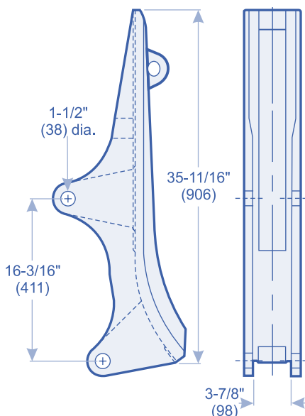
198-78-21390HX 148.0 lbs. (67.1 kgs.)
