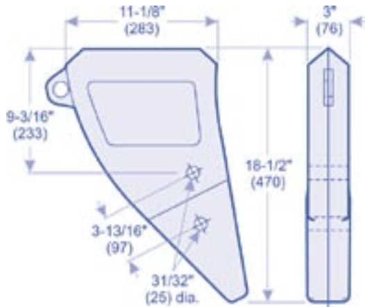
17M-78-21360HX 112.0 lbs. (50.8 kgs.)
