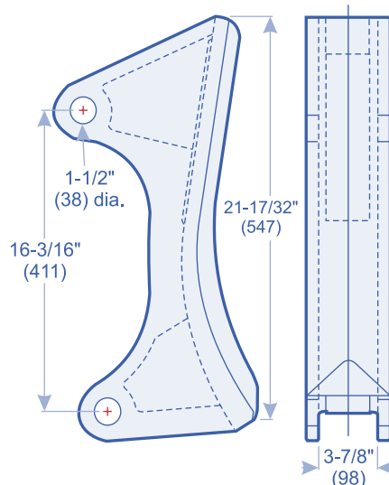
198-78-21330HX 86.0 lbs. (39.0 kgs.)
