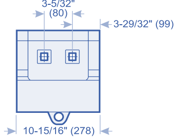
421-815-1221NR 42.0 lbs. (19.0 kgs.) Requires (2) A78-312 plow bolt assemblies each
