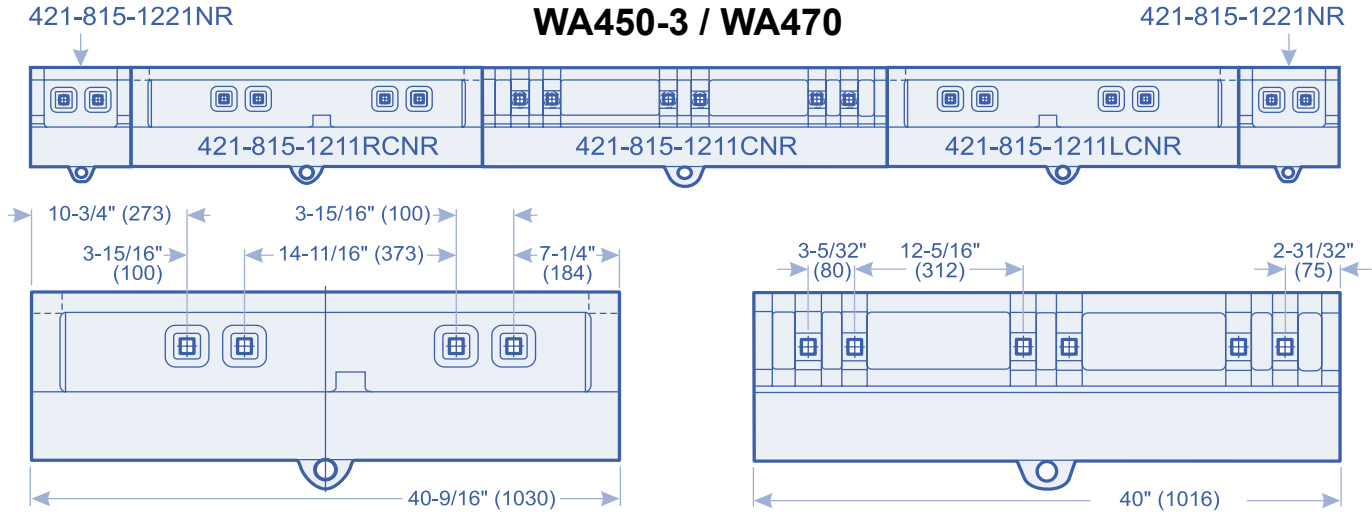
421-815-1211RCNR (RH shown) 421-815-1211LCNR (LH opposite) 110.0 lbs. (50.4 kgs.) Requires (4) A78-312 plow bolt assemblies each
