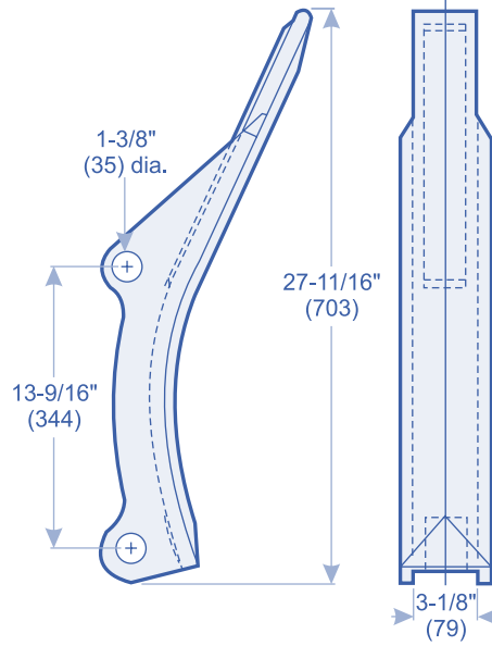
195-78-21580HX 51.7 lbs. (23.5 kgs.)
