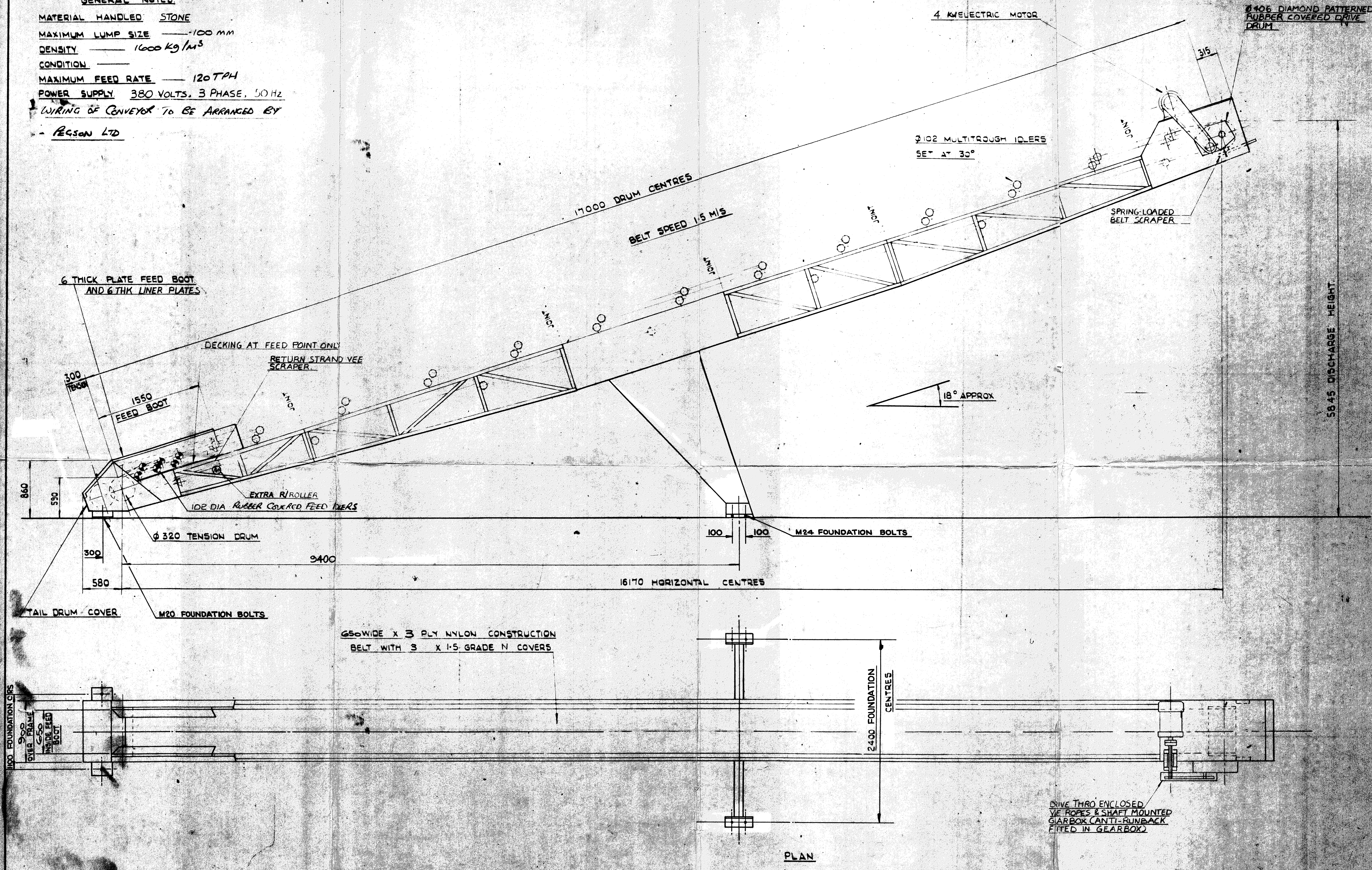
GENERAL ARRANGEMENT OF 17 METRE CENTRES X 650 WIDE SPECIAL T.B.C. TYPE N.F.M.
