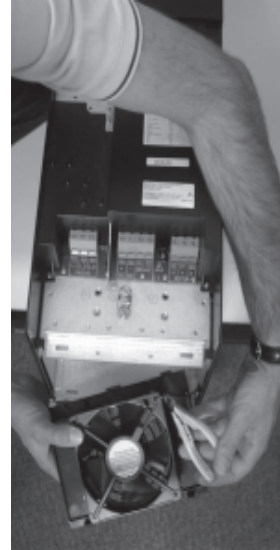
3. Cut the cable with a diagonal cutting nipper.
