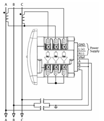
DELTA with PTs 3 Phase, 3-wire
