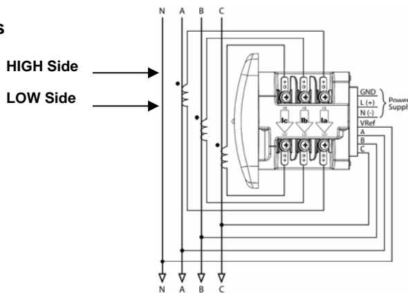
WYE Direct 3 Phase, 4-wire
