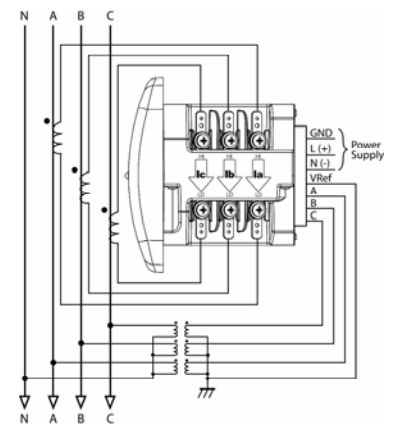
WYE with PTs 3 Phase, 4-wire
