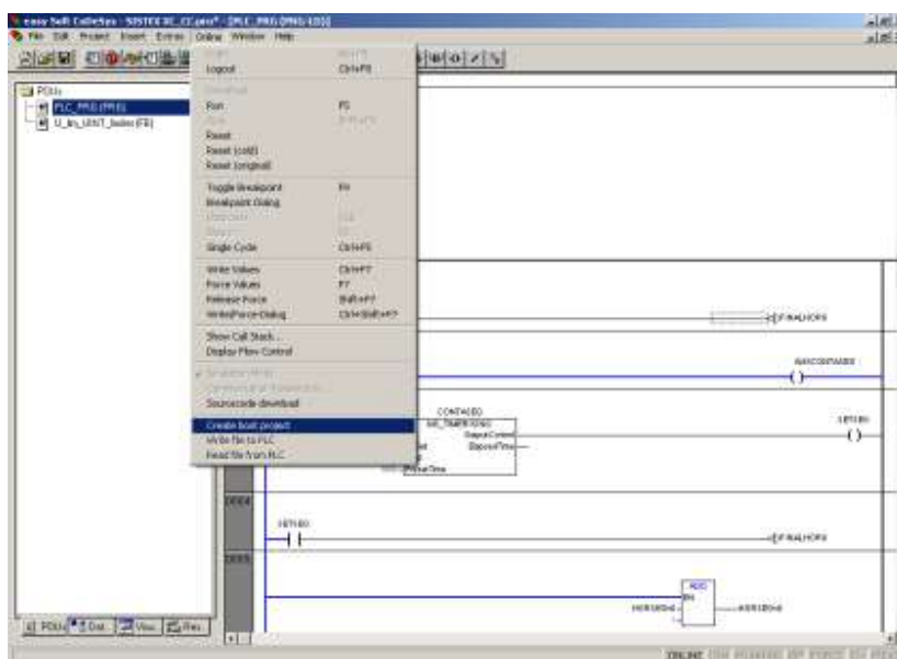
Figure 74 - PLC download completed
