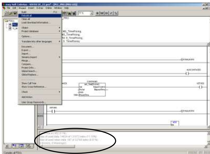
Figura 71 – Verification of the CLP programming
