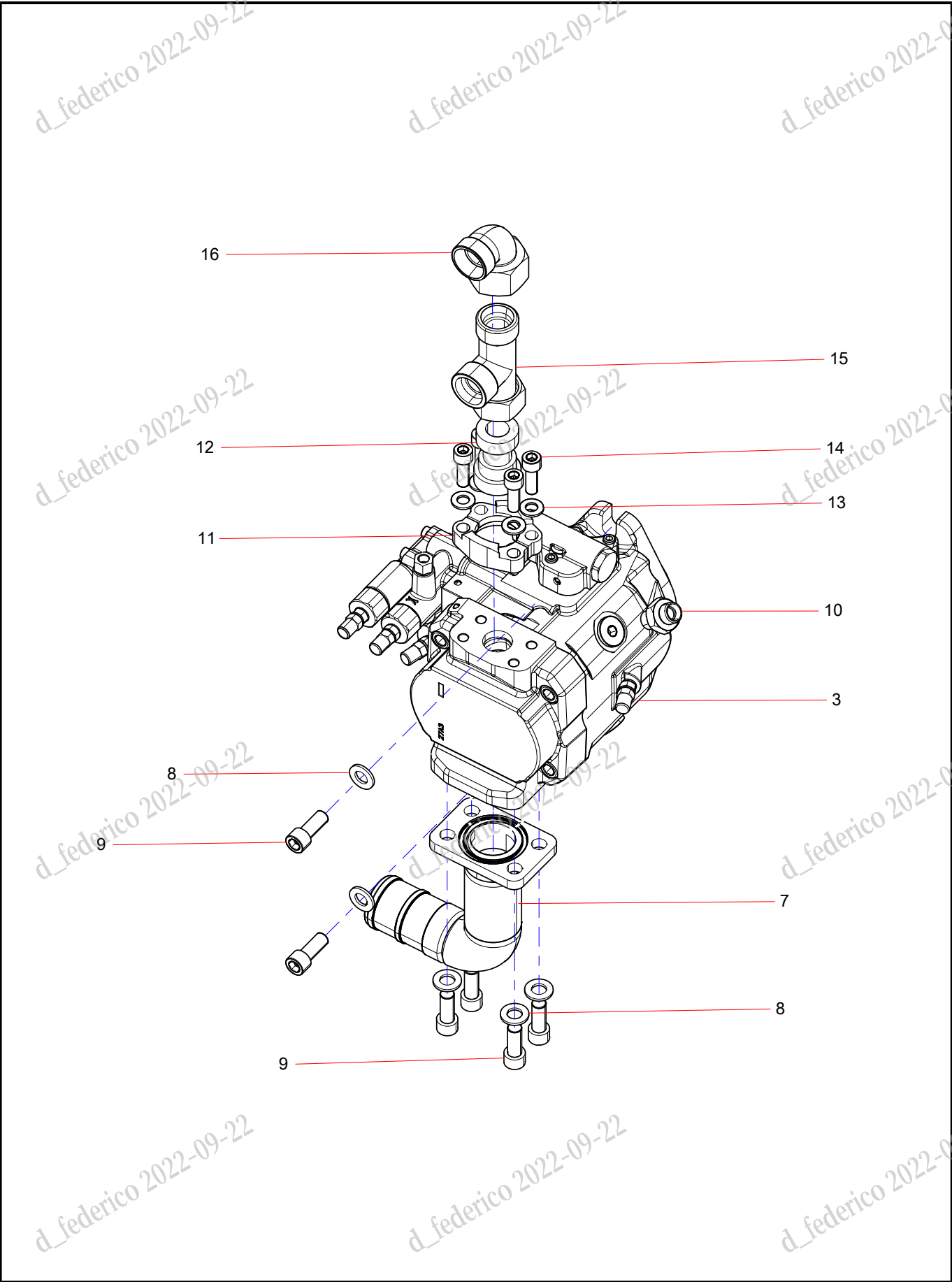
7-6 Slewing device
