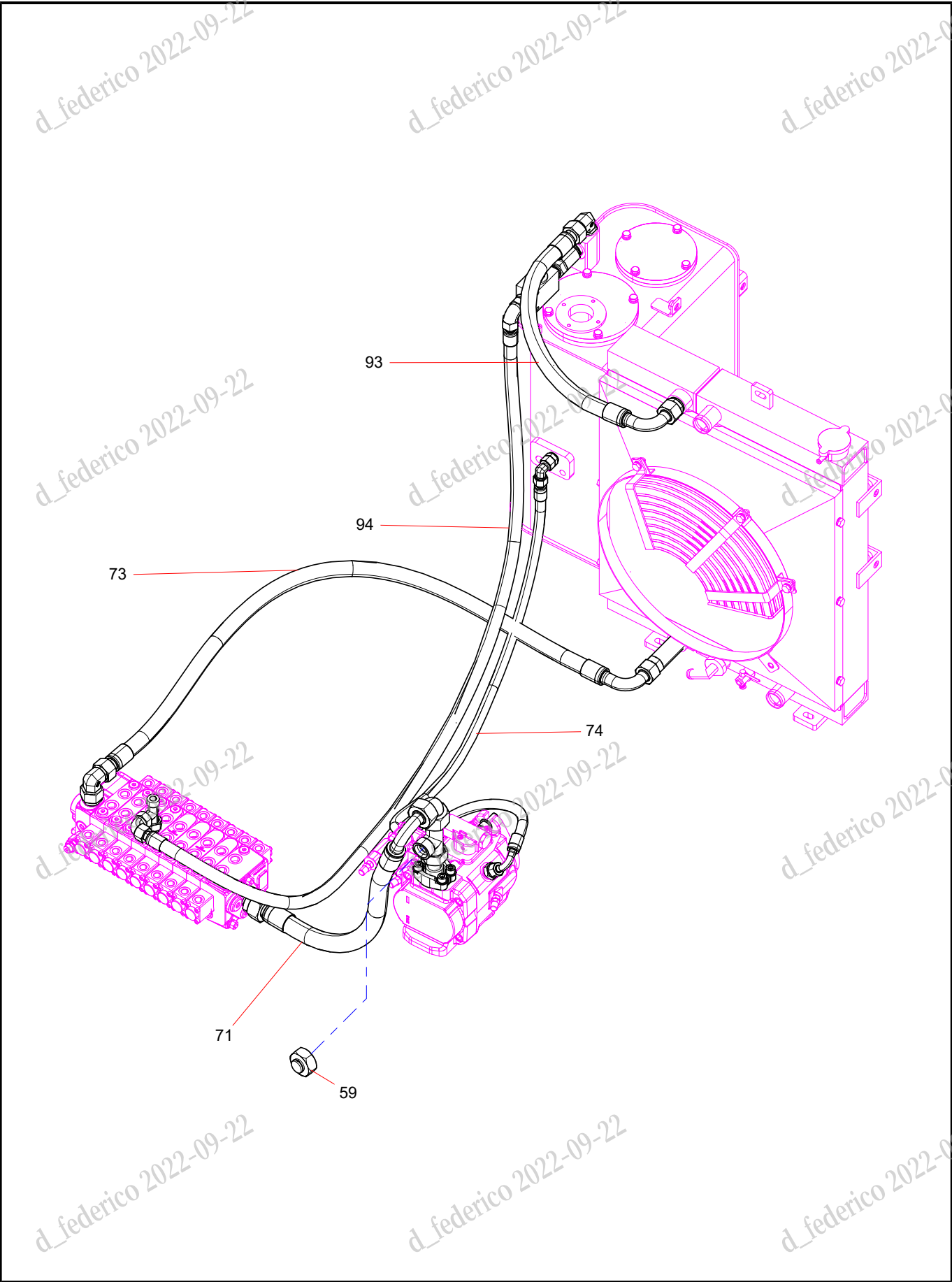
7-18 Slewing device
