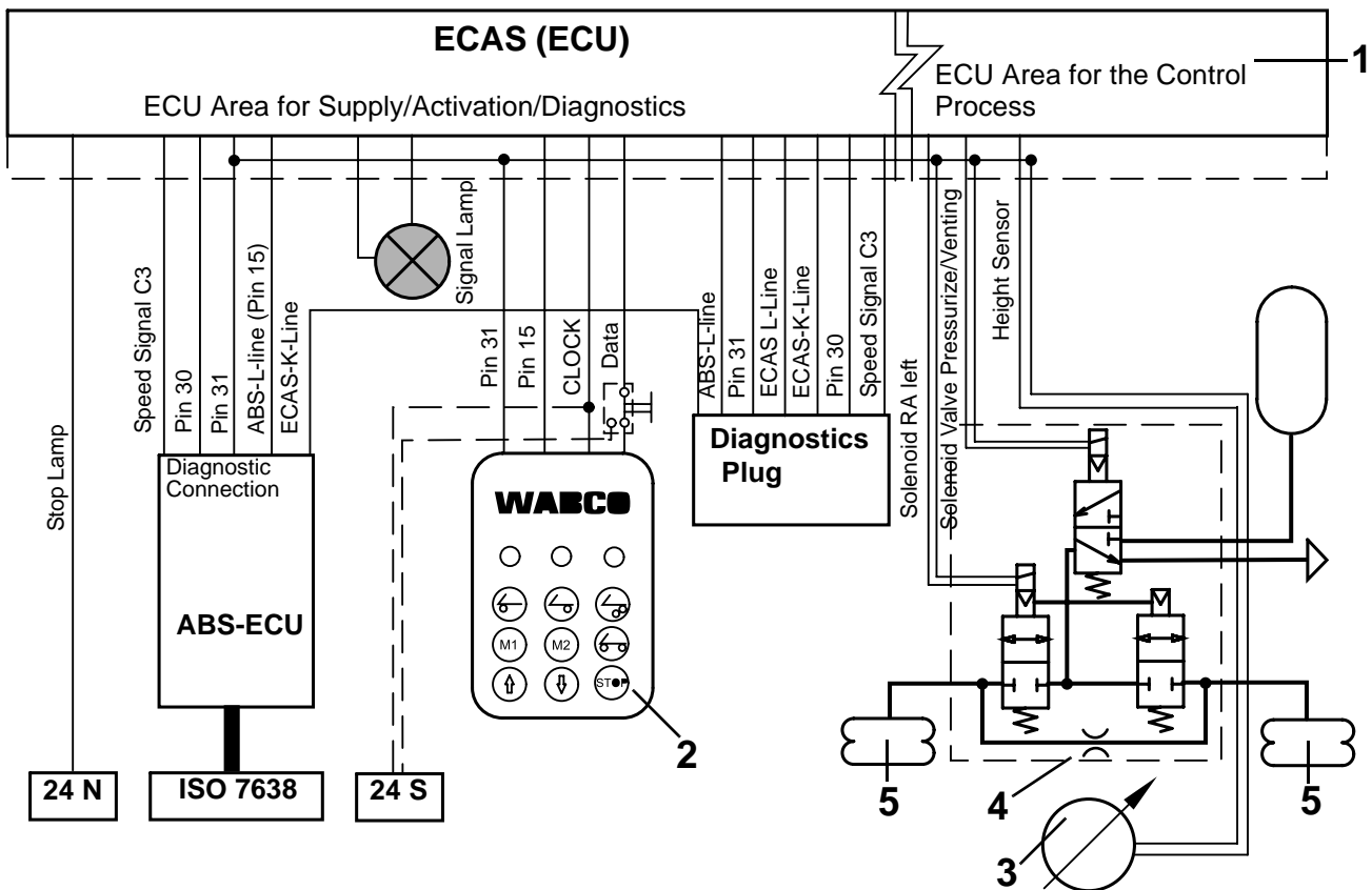
1 ECU 2 Remote Control 3 Height Sensor 4 Solenoid Valve 5 Bellow
