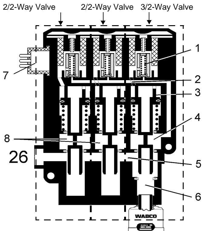
Fig. 26 Cross-Section of an ECAS Solenoid Valve with Spring-Returned Sliding Valves for the Leading Axle or the Main Axle Portion (Solenoid Block)
