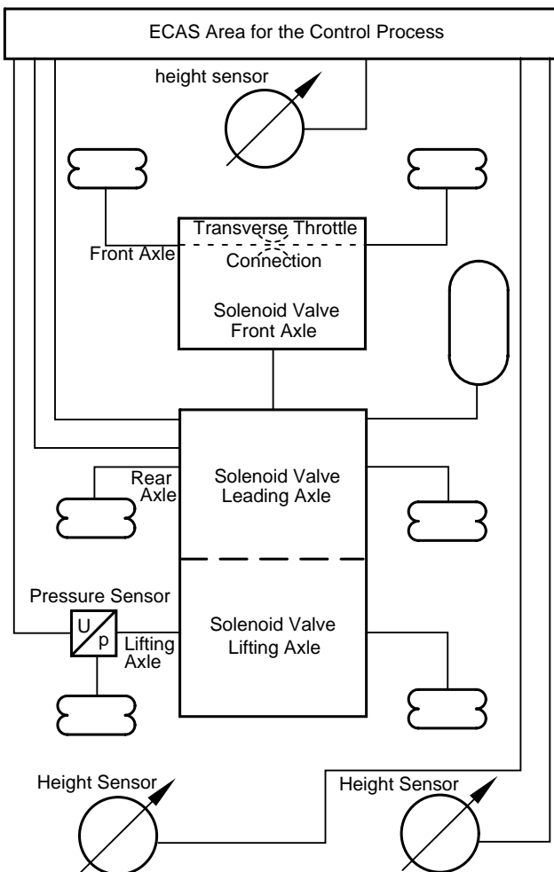
Fig. 10 Vehicle with 2-Point Control on Rear Axle
