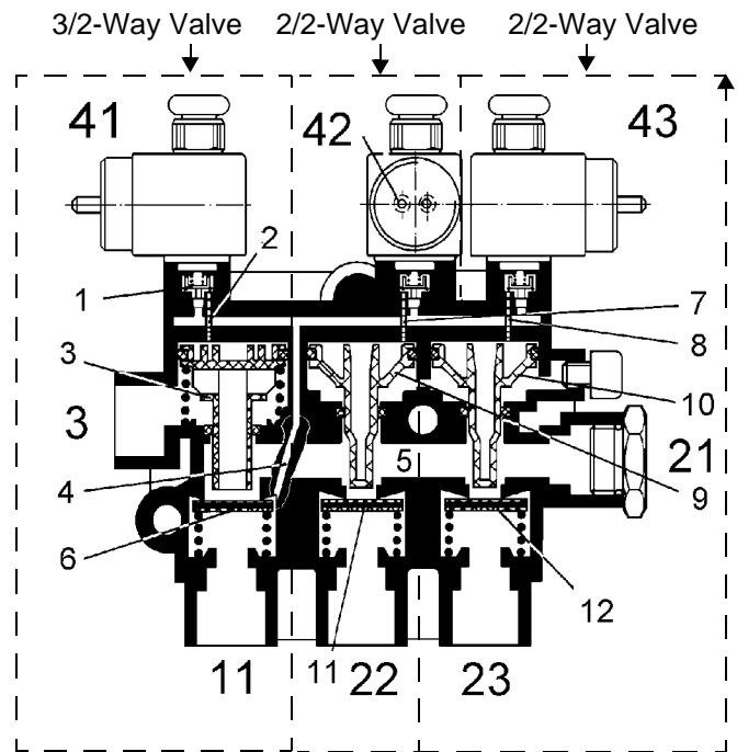
Fig. 25 Cross-Section of an ECAS Solenoid Valve with Spring-Returned Seat Valves for the Leading Axle (Individual Solenoids)
